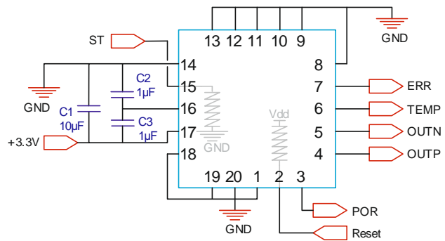
Figure 40: Proximity circuit & internal pull-up/down
