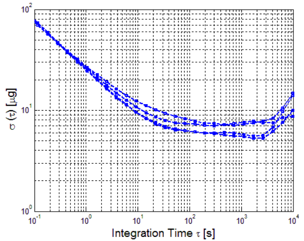
Figure 38: Allan Variance
