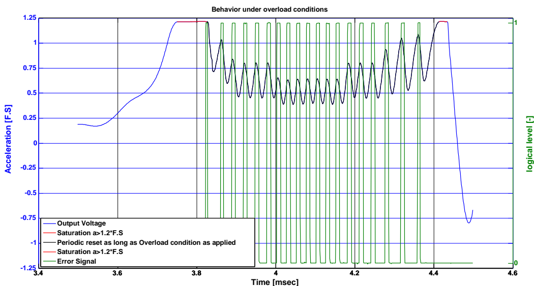
Figure 44: Overload Behavior
