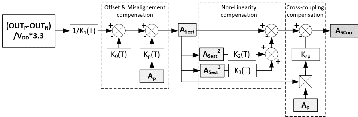
Figure 49 : Recommended compensation scheme
