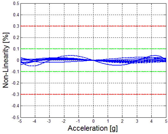
Figure 21 : Non-linearity under vibration
