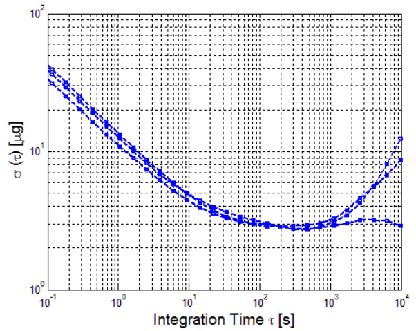
Figure 26: Allan Variance
