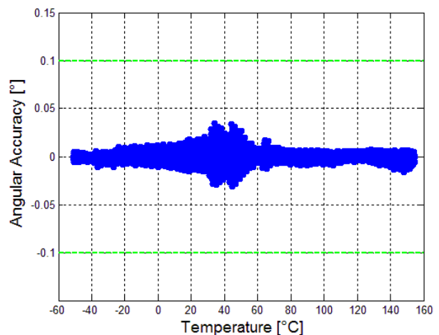
Figure 51: Angular accuracy over temperature of a TS1002TA sensor
