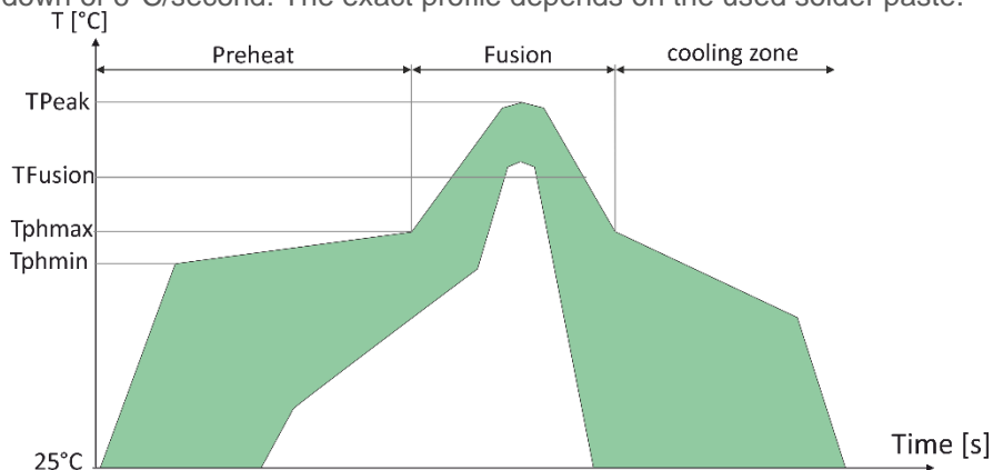
Figure 48: Soldering Temperature Profile
