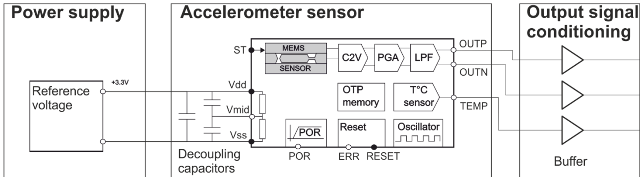
Figure 46: Block diagram
