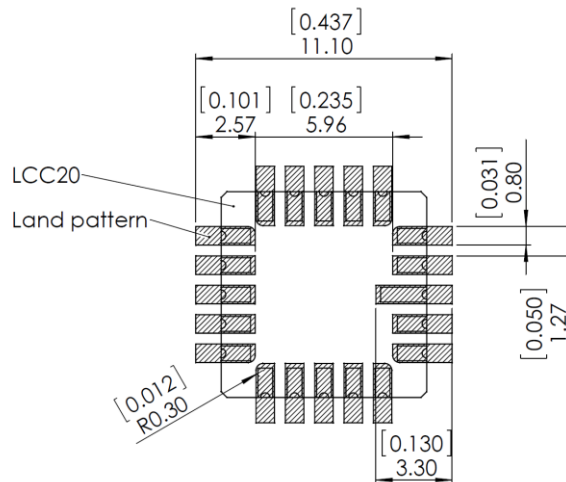
Figure 47 : LCC20 land pattern recommendation (unit are mm/[inch])
