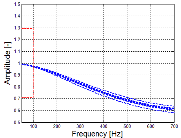
Figure 12 : Frequency response
